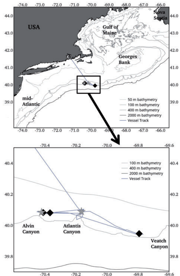
Figure 1. Data collection sites. Stars denote bongo sampling sites and diamonds denote 4SBT hauls.
